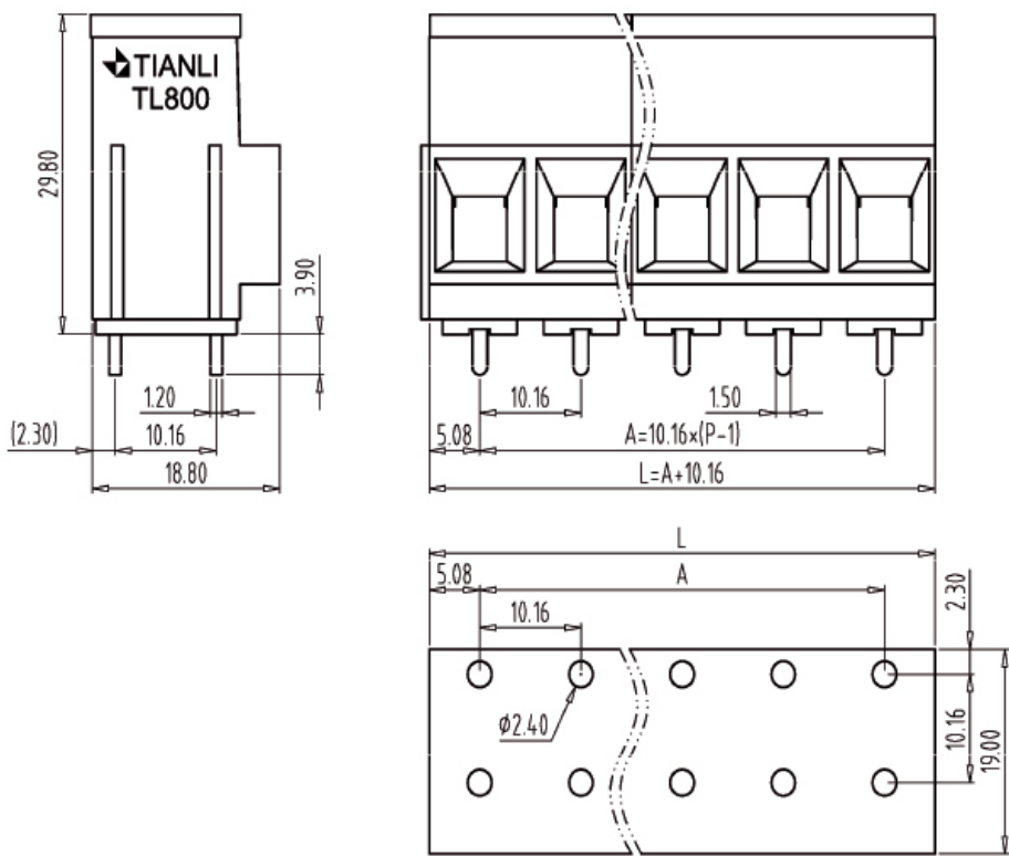
PCB Layout
